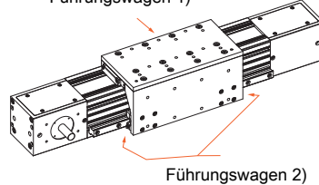
LM5...Z...L/R
